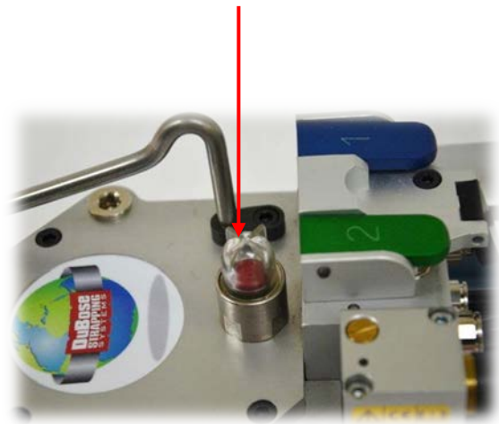
OPTIONAL WELD TIME INDICATOR
